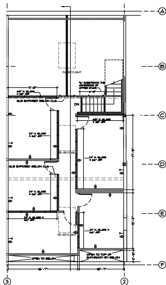
MEZZANINE LEVEL
