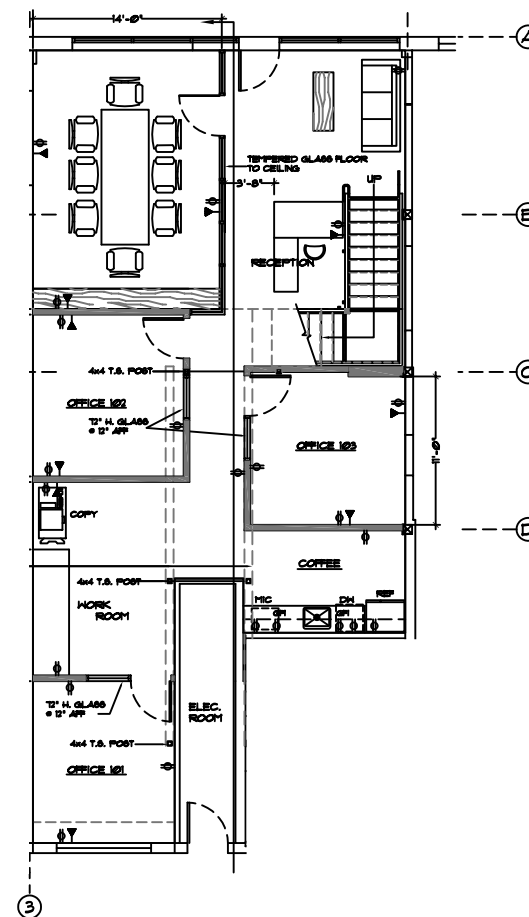
GROUND FLOOR LEVEL
